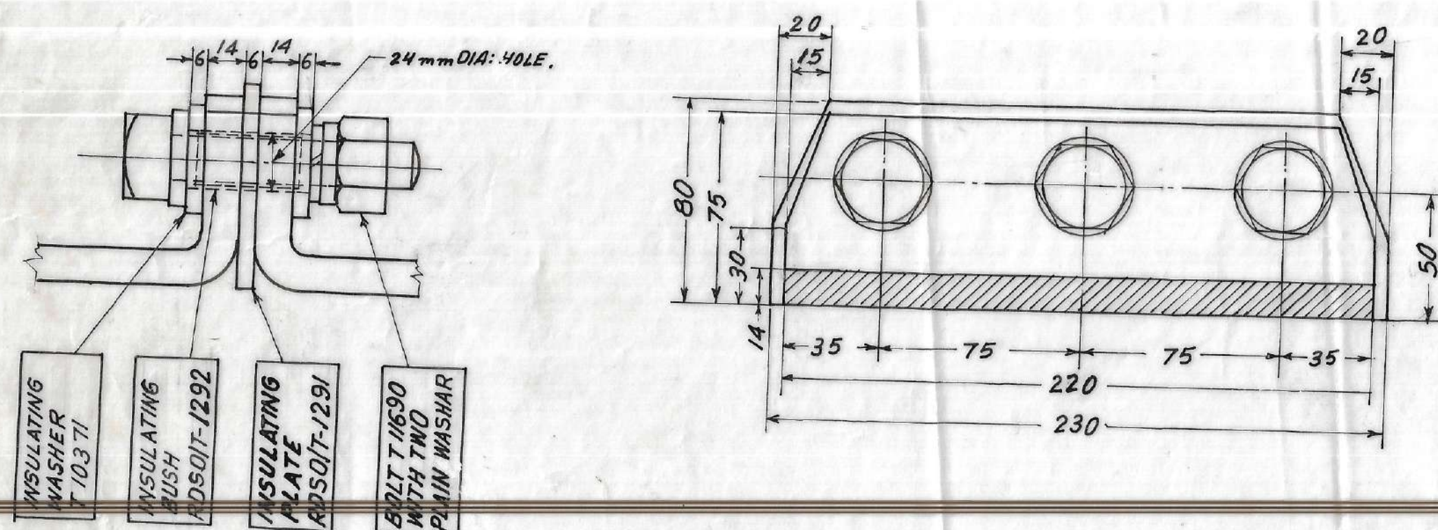
DETAIL OF INSULATED JOINT
